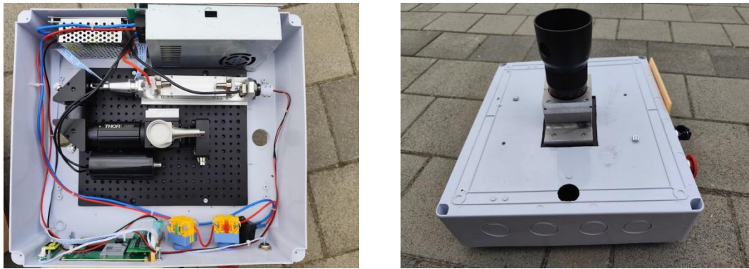
Figure 2. Photos of the internal system assembly (left) and the optics (right).
